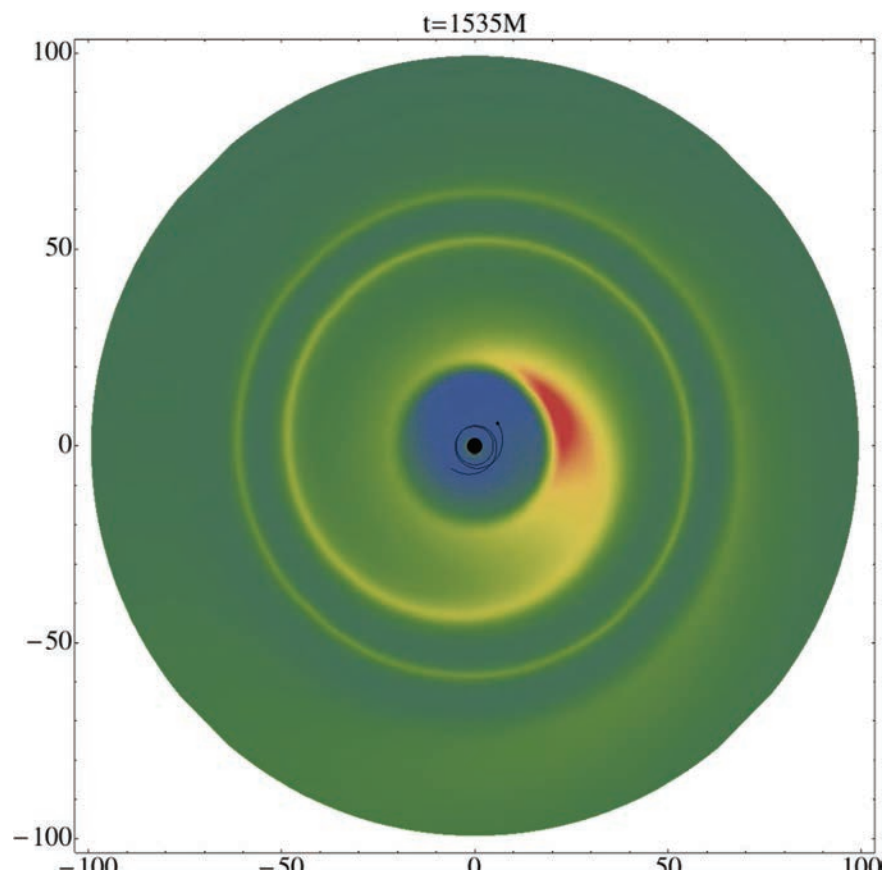
Equatorial snapshot of the scalar field produced by a scalar charge in orbit around a black hole. The central black dot shows the black hole. The smaller black dot shows the current location of the scalar charge and the line trailing it shows a part of the previous trajectory. Notice the spiral pattern in the wave traveling outwards.
