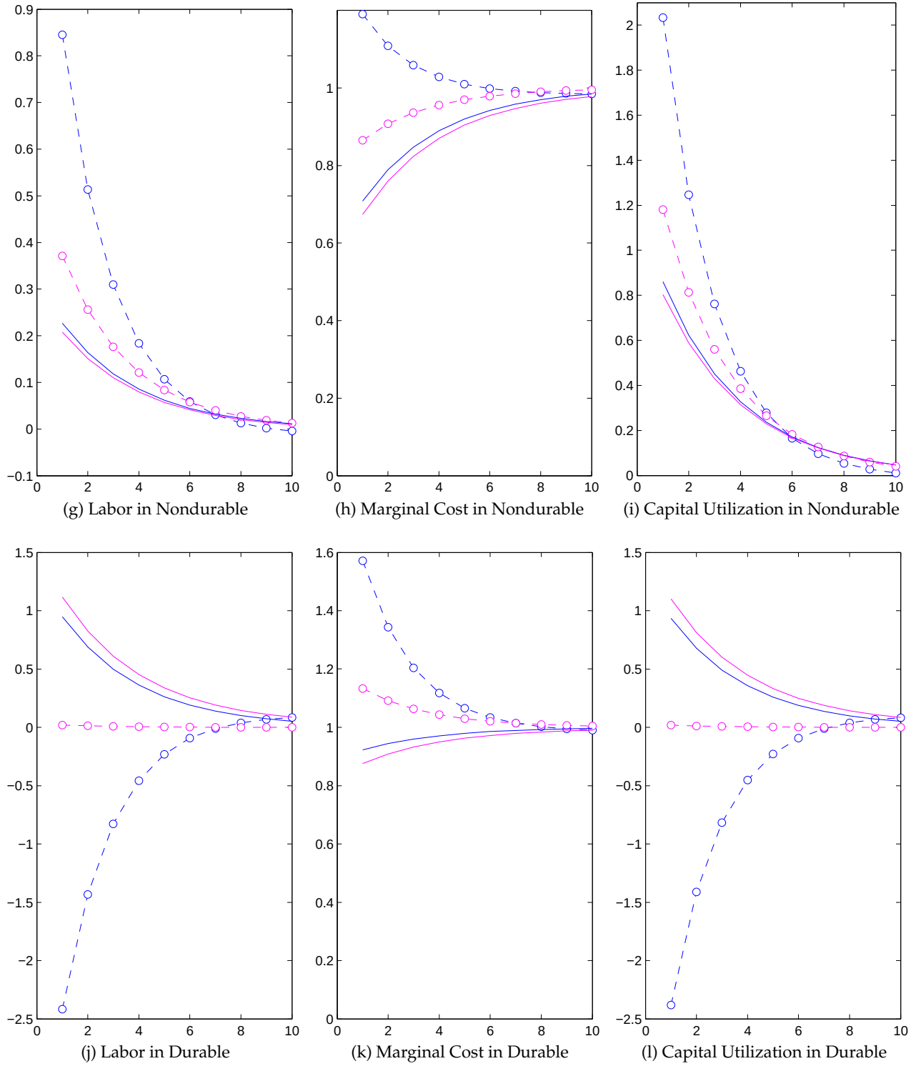
Figure 2: IRFs with Variable Capital Utilization ( Continued )
