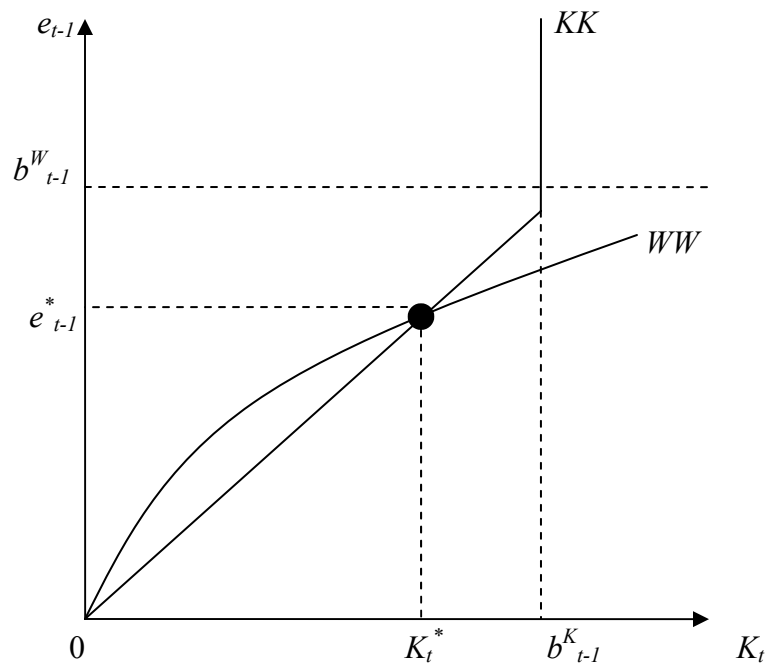
Figure 6: Reaction Functions e^*_{t-1} < b^W_{t-1} , K_t^* < b^K_{t-1}
